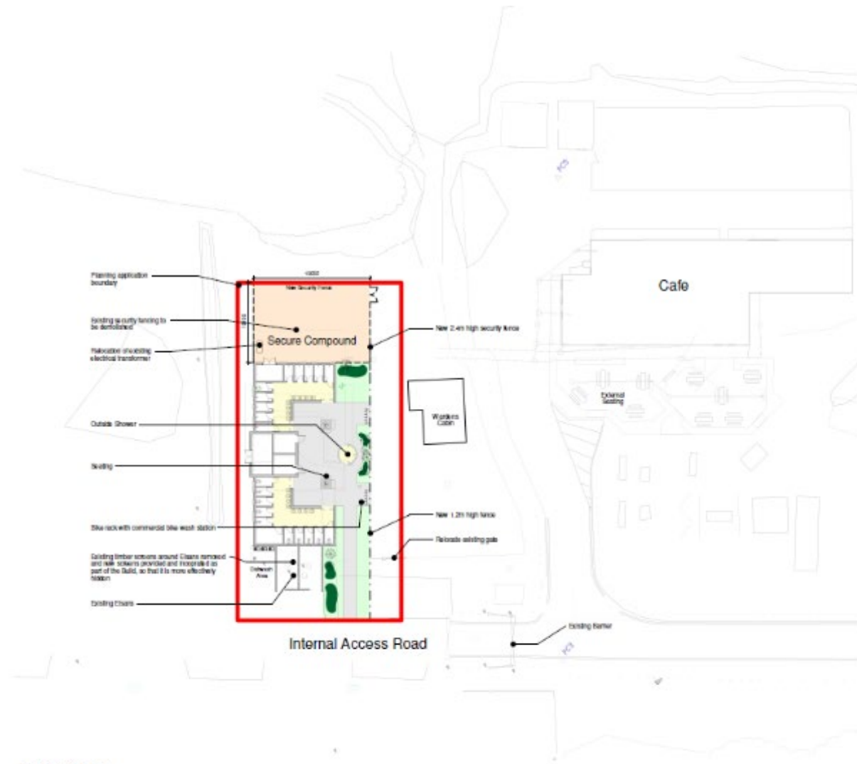
Proposed Plan 1 : 200
